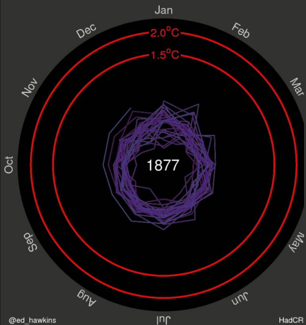
Global temperature change (1850–2016)
