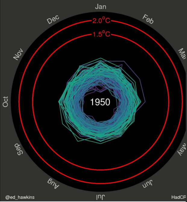
Global temperature change (1850–2016)
