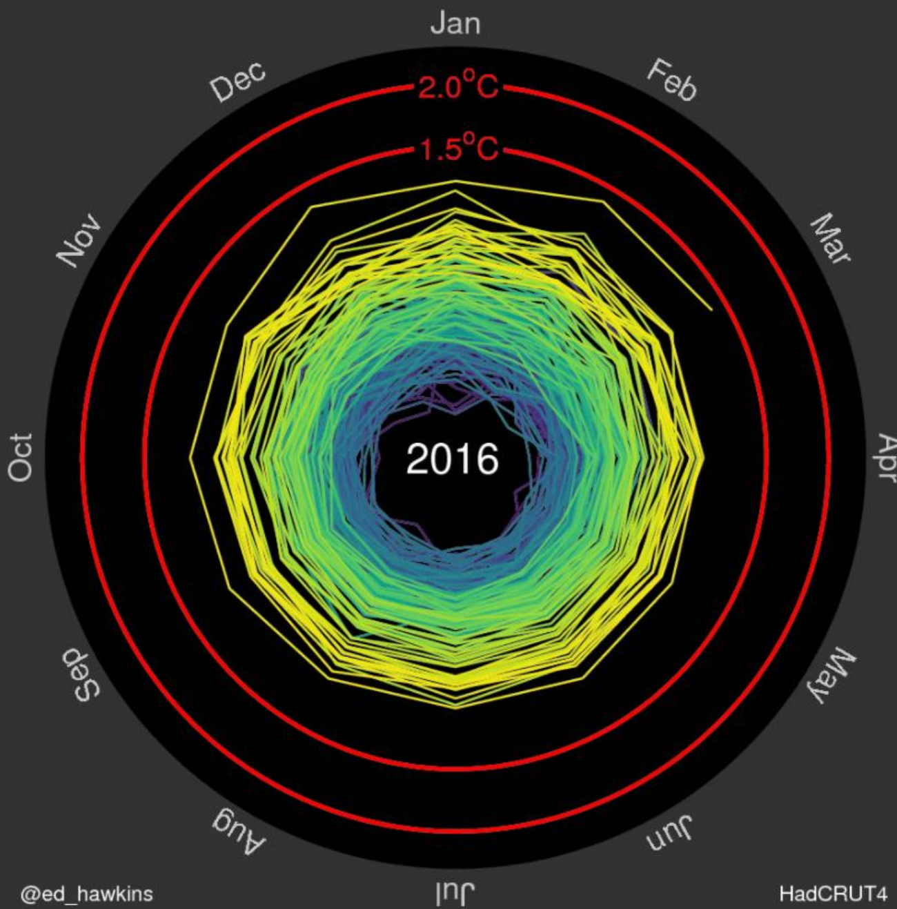
Global temperature change (1850–2016)
